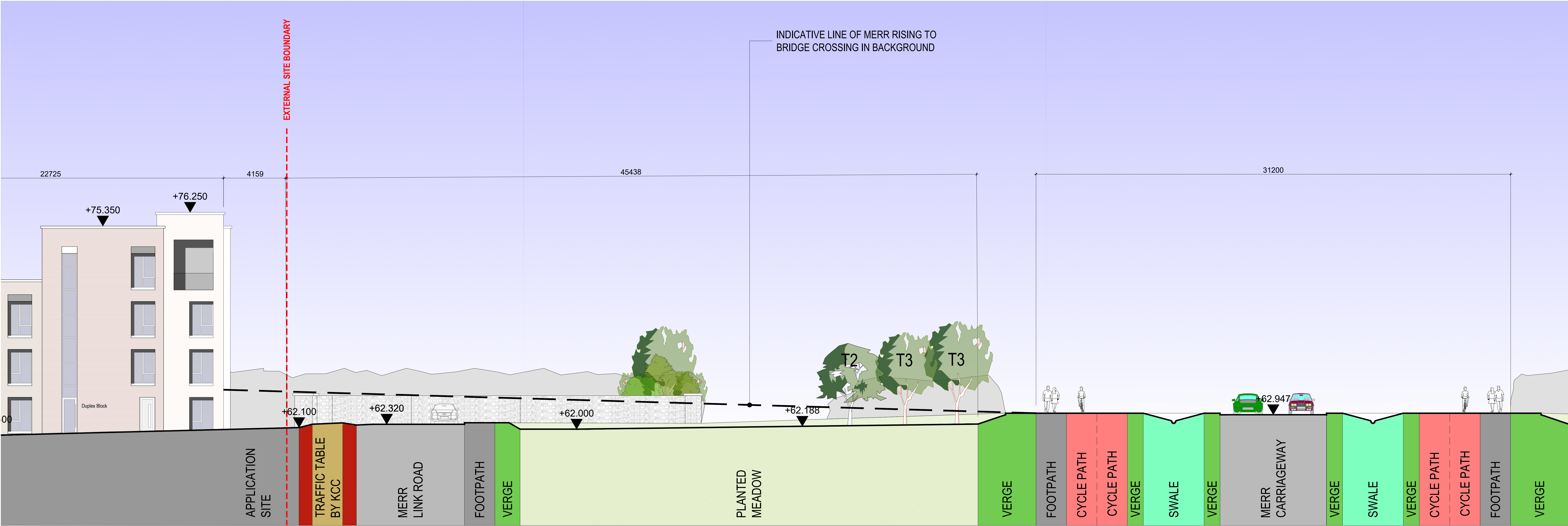
MERR CONTEXT ELEVATION 2-2 Scale 1:100
